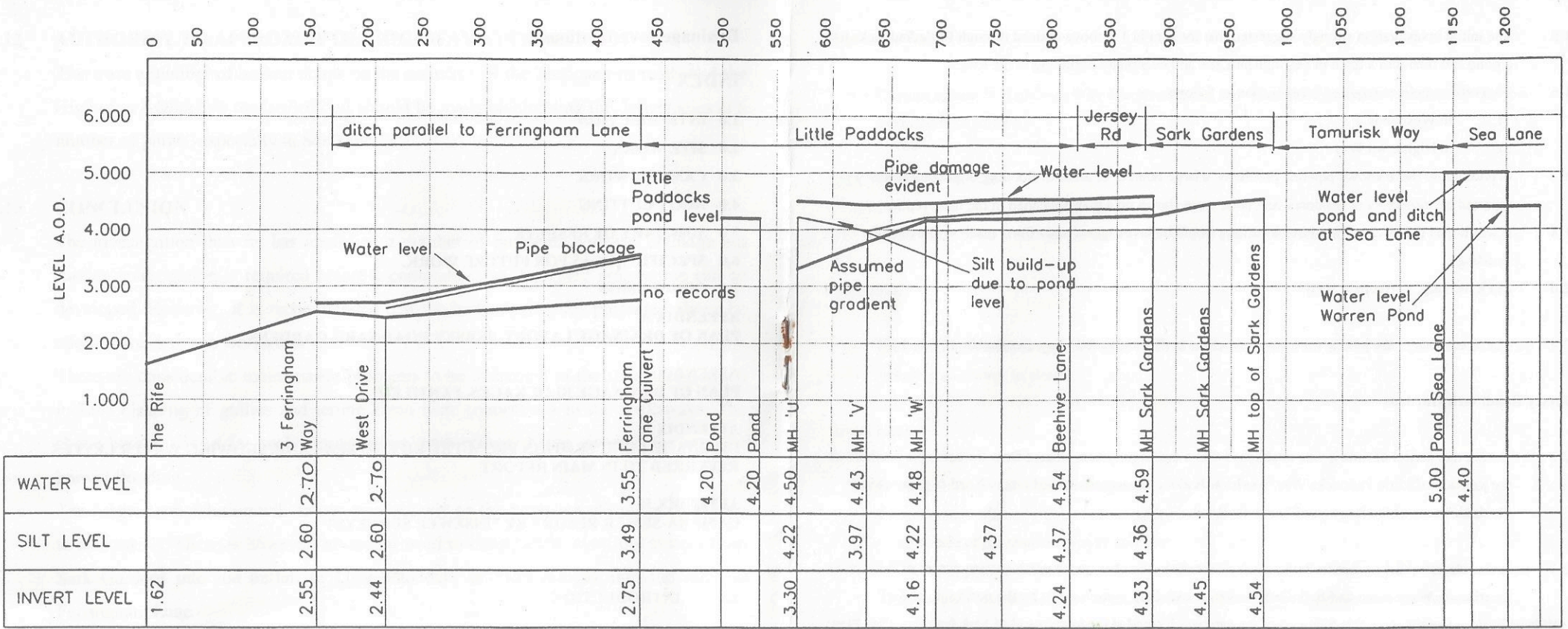
DRAINAGE LONG SECTION FROM THE RIFE - FERRINGHAM LANE - SARK GARDENS - SEA LANE SCALE 1:100 VERTICAL, 1:500 HORIZONTAL
